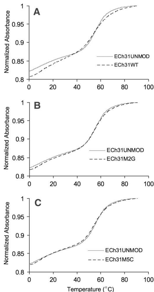
Figure 2. Representative normalized UV melting curves of the modified RNAs compared to the unmodified RNA, taken in 15 mM NaCl, 20 mM sodium cacodylate, 0.5 mM Na 2 EDTA (pH 7.0), are shown. The melting curves for the unmodified RNA (ECh31UNMOD, solid gray lines in panels A–C) are compared to those for the modified RNAs (dashed lines): (A) ECh31WT, (B) ECh31M2G, and (C) ECh31M5C. All of the melting curves were normalized at 95 °C and absorbance measurements were taken at 280 nm.
