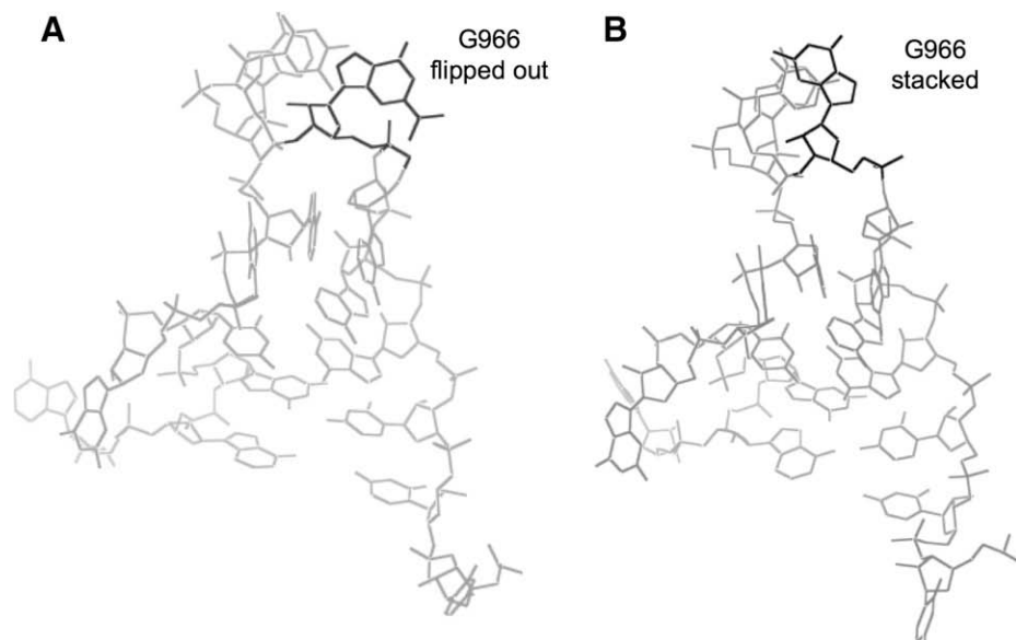
Figure 4. Structures of h31 showing the flipped out (A) and stacked (B) conformations of residue G966 (PDB accession IDs—2J00 15 and 1FJF 22 ).
