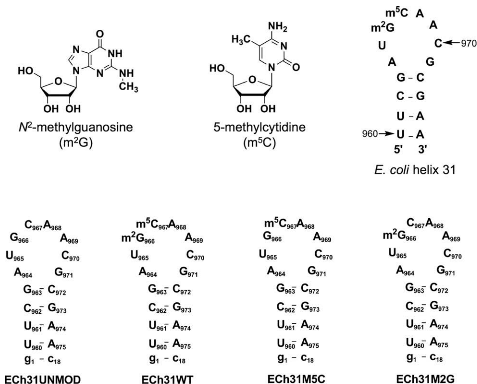
Figure 1. The structures of N 2 -methylguanosine ( m 2 G) and 5-methylcytidine ( m 5 C) are shown. Secondary structure representations of E. coli helix 31 of the small subunit ribosomal RNA with indications of the modification sites and the synthetic RNA hairpins derived from residues 960–975 are shown (unmodified (ECh31UNMOD), fully modified (wild-type or ECh31WT, containing m 2 G 966 and m 5 C 967 ), m 5 C 967 singly modified (ECh31M5C), and m 2 G 966 singly modified (ECh31M2G)). The terminal G–C base pair (g 1 –c 18 ) was added to stabilize the short stem region.
