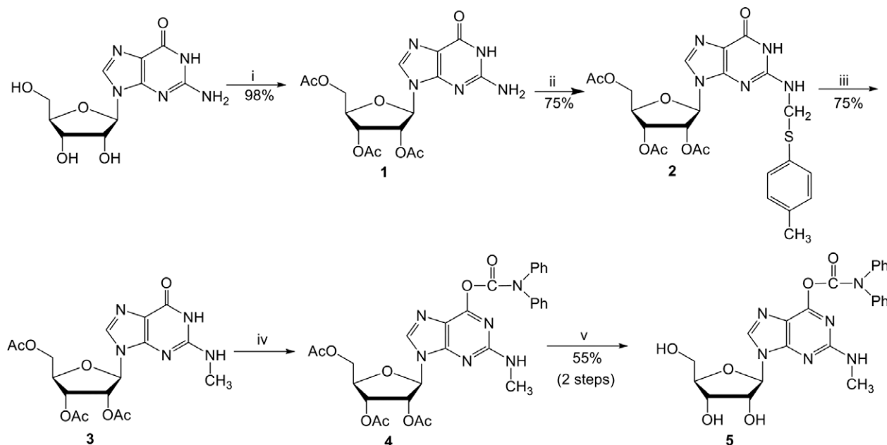
Scheme 1. Synthesis of the 6-O-DPC-2-N-methylguanosine 5 : (i) acetic anhydride, DMAP, Et 3 N, acetonitrile, 0.5 h; (ii) p -thiocresol, acetic acid, formaldehyde, ethanol, reflux; (iii) NaBH 4 , DMSO, 100 °C; (iv) DPCl, diisopropylethylamine, pyridine; (v) (a) 2 M NaOH, 20 min; (b) acetic acid.
