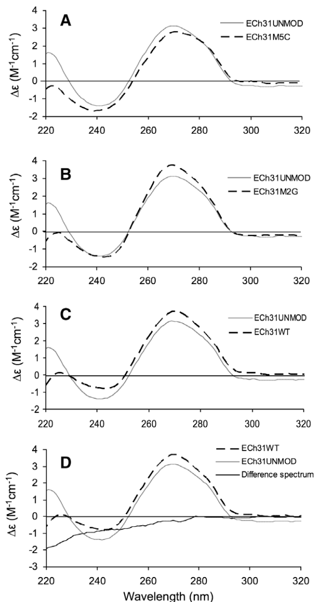
Figure 3. CD spectra of the modified and unmodified RNA constructs are shown. Each spectrum is an average of five scans. The CD spectrum of the unmodified analogue (ECh31UNMOD, solid gray line) is shown in panels A–C with overlays (dashed lines) of the ECh31M5C (A), ECh31M2G (B), and ECh31WT (C) RNAs. The molar ellipticities are normalized to RNA concentrations. The total difference spectrum (ECh31M5C + ECh31M2G – ECh31UNMOD – ECh31WT) is shown in panel D (solid black line).
